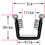
Y691P Flexible Polypropylene Pile Lining Rubber-Covered
