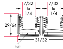
Y583 Rigid Polypropylene Pile Lining Uncovered
