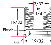
Y582 Rigid Polypropylene Pile Lining Uncovered
