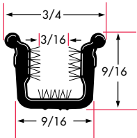
Y630P Flexible Polypropylene Pile Lining Rubber-Covered
