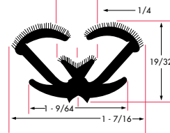
AS1720 Flexible Flocked Lining All-Rubber 75001374 96"
